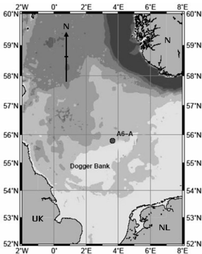
Figure 1: Location of A6-A-Kolskaya complex in the German Sector of the North Sea. Lightest grey bathymetry region delineates 30 m contours. Map projection: Mercator.
